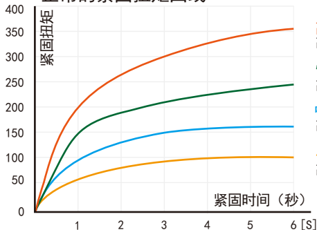
[Nm] 正常的紧固扭矩曲线
