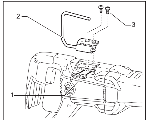
▶ 1. 方形螺母 2. 挂钩 3. 螺丝
